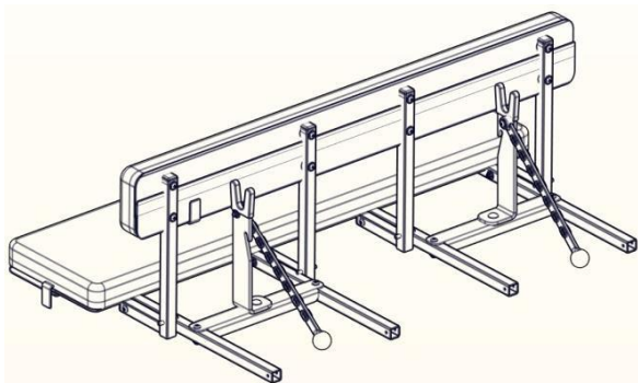
ASSEMBLED VIEW
